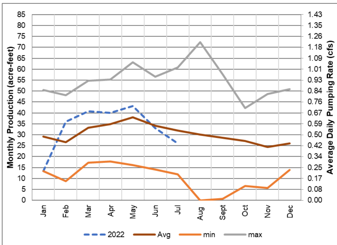
Figure 3. Monthly well extraction volume from CCSD San Simeon basin wells in 2022 and average, minimum, and maximum monthly well extraction volumes with average daily pumping rates for the period from 2012 through July 2022.
