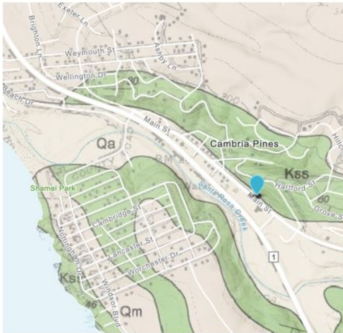
Figure 4: Regional Geologic Map
