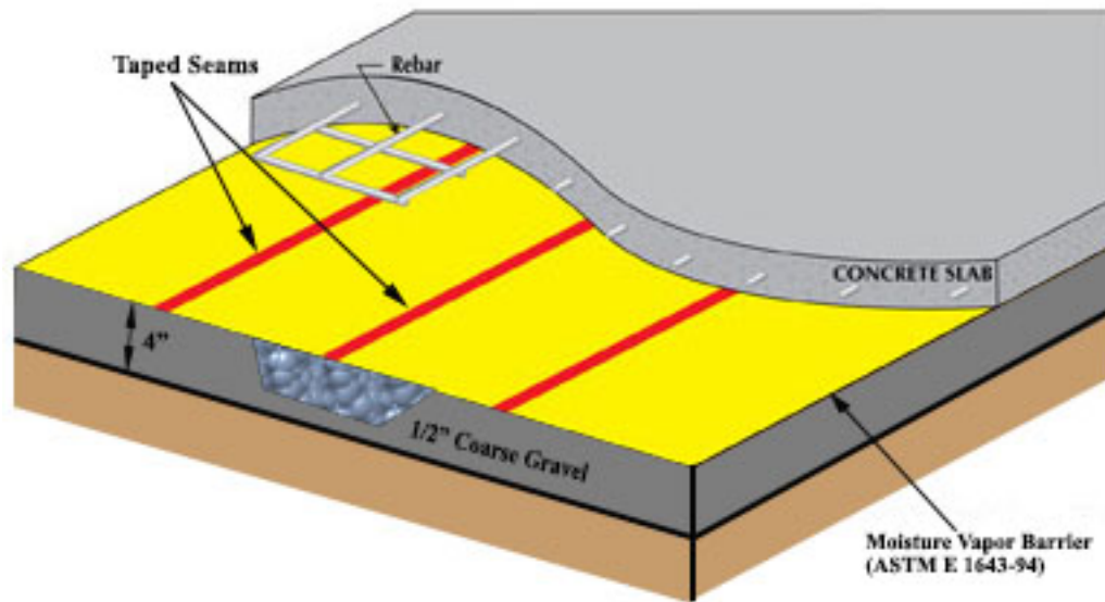
Figure 6: Sub-Slab Detail
